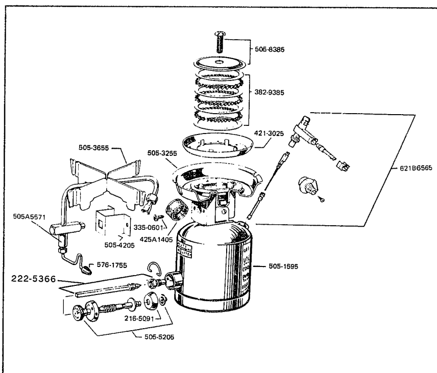
MODEL 505A SINGLE BURNER – CAMP STOVE
